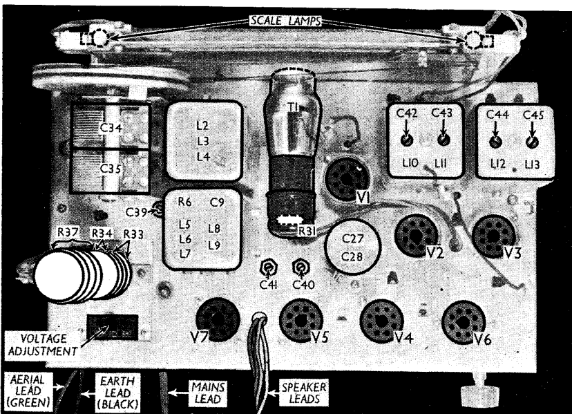
Plan view of the chassis. The adjustment screws of the trackers C39, C40 and C41 are indicated. Note the positions of R33, R34 and R37.
